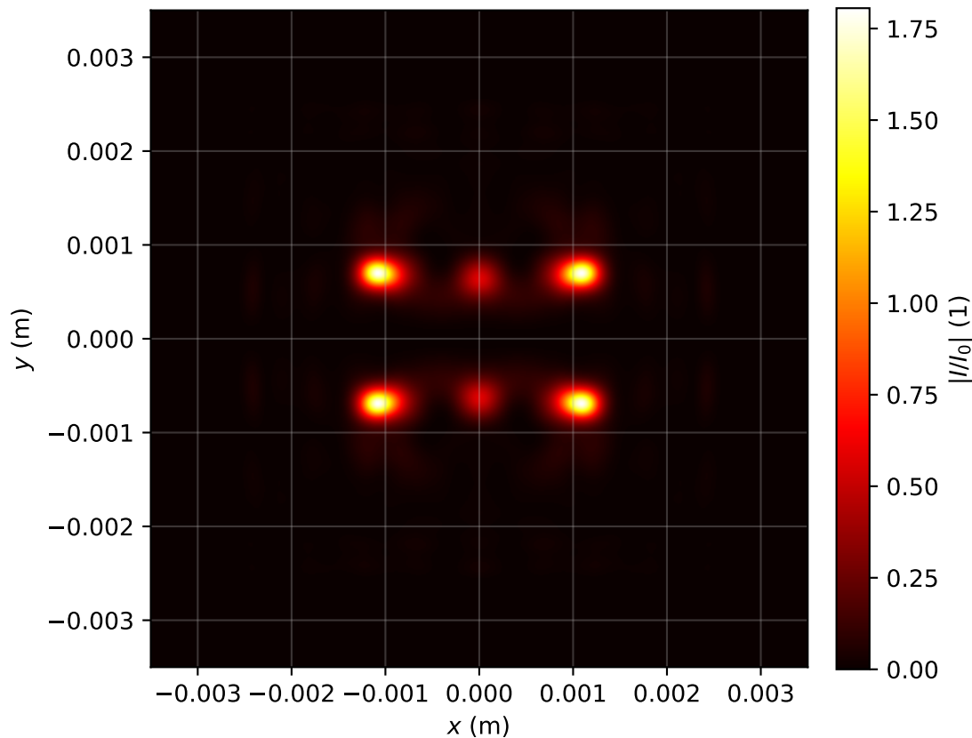
Intensity profile I(x, y, z = 2.149)/I_0 , P_{in}=7.0P_{cr} , artificial time
